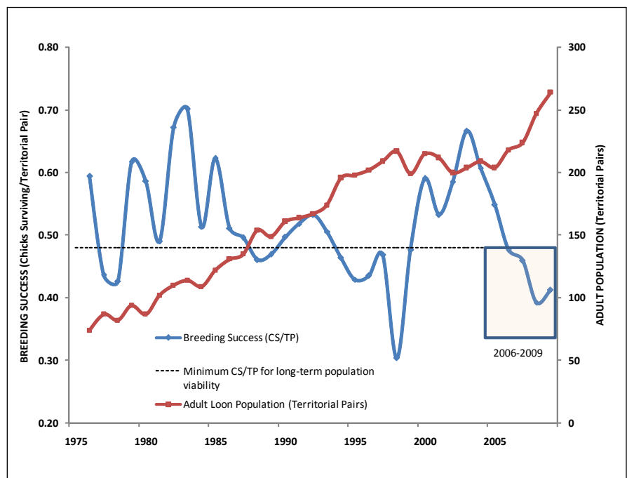
Figure 2. Loon Breeding Success (chicks surviving per territorial pair) and Adult Population Size, 1975-2009.
